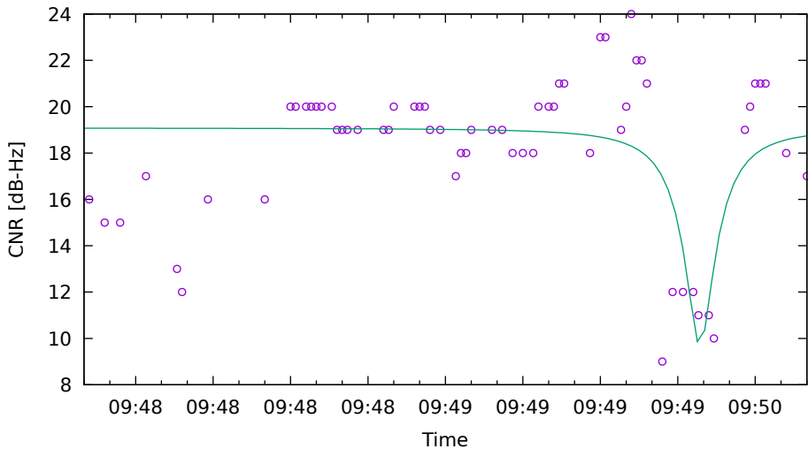
CNR fit for C11 on HuaweiP40 - drive 17 (DOY262)
