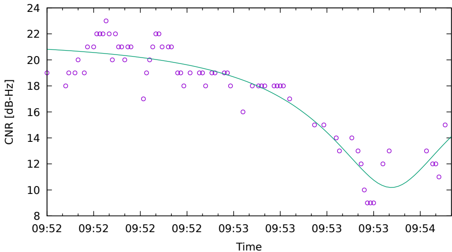
CNR fit for C11 on HuaweiP40 - drive 19 (DOY262)
