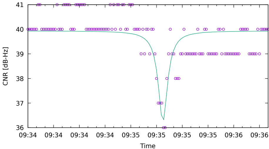
CNR fit for C16 on HuaweiP40 - drive 10 (DOY262)
