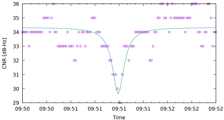
CNR fit for C16 on HuaweiP40 - drive 18 (DOY262)
