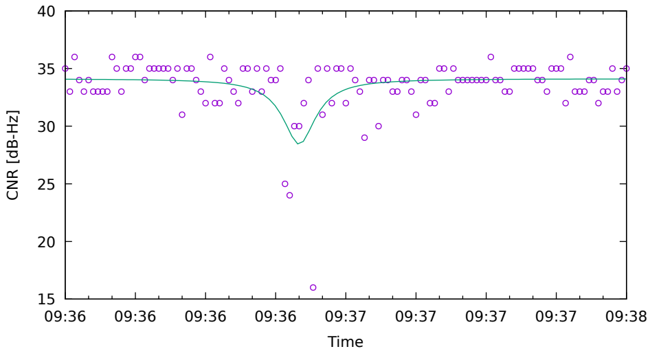
CNR fit for C27 on HuaweiP40 - drive 11 (DOY262)
