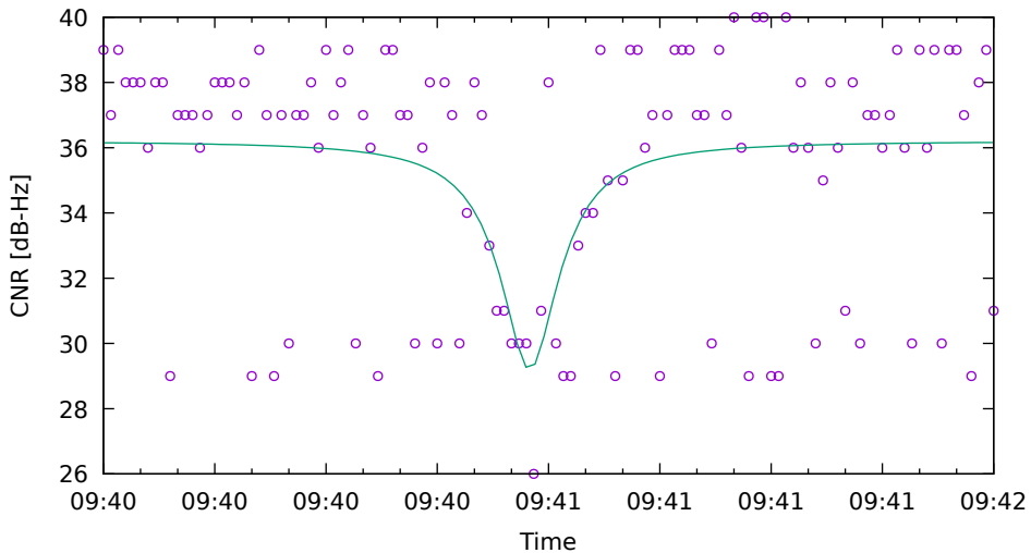
CNR fit for C27 on HuaweiP40 - drive 13 (DOY262)
