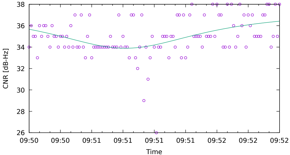
CNR fit for C27 on HuaweiP40 - drive 18 (DOY262)
