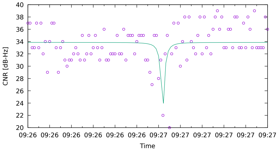
CNR fit for C27 on HuaweiP40 - drive 6 (DOY262)
