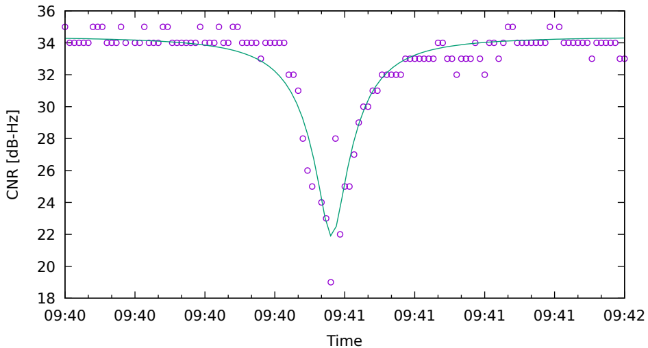
CNR fit for G01 on HuaweiP40 - drive 13 (DOY262)
