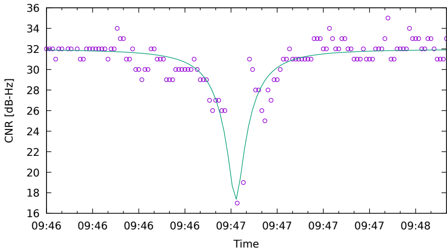
CNR fit for G01 on HuaweiP40 - drive 16 (DOY262)
