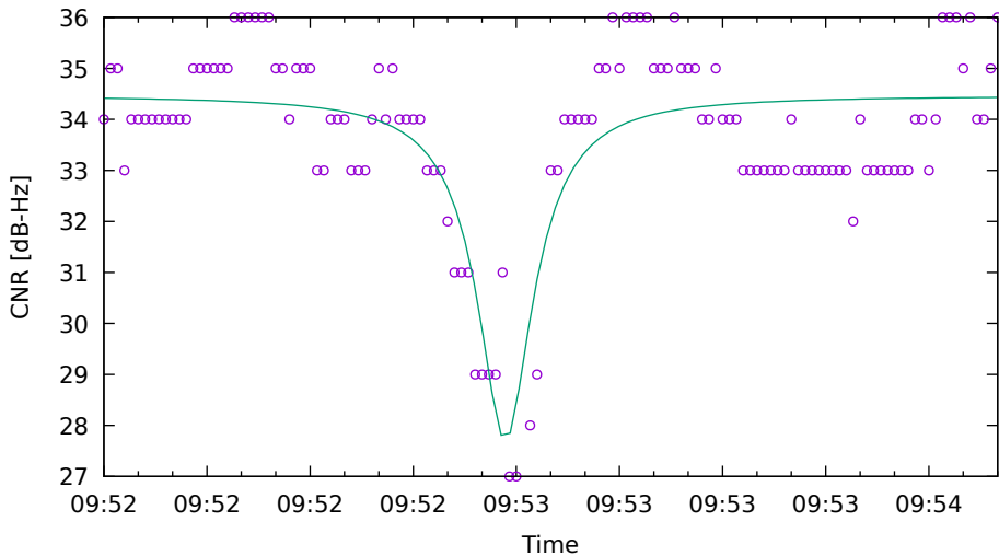
CNR fit for G01 on HuaweiP40 - drive 19 (DOY262)
