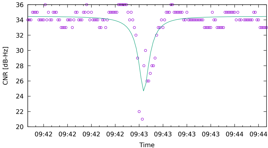
CNR fit for G03 on HuaweiP40 - drive 14 (DOY262)
