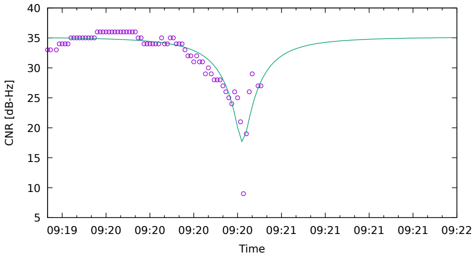
CNR fit for G03 on HuaweiP40 - drive 3 (DOY262)
