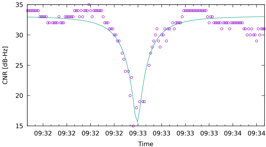
CNR fit for G03 on HuaweiP40 - drive 9 (DOY262)
