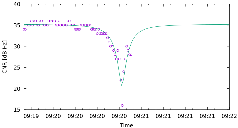
CNR fit for G04 on HuaweiP40 - drive 3 (DOY262)
