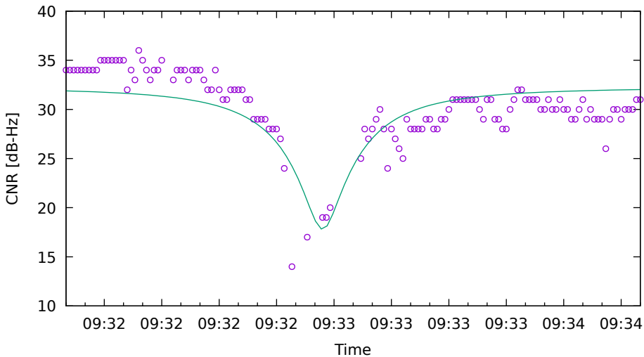
CNR fit for G04 on HuaweiP40 - drive 9 (DOY262)
