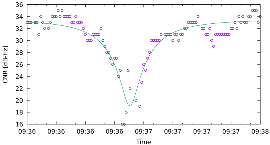
CNR fit for G17 on HuaweiP40 - drive 11 (DOY262)
