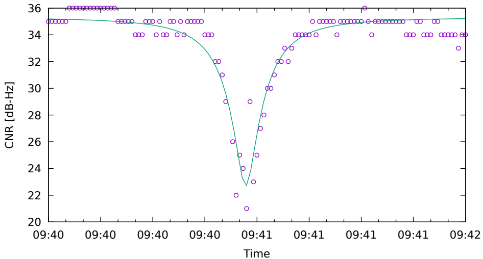
CNR fit for G17 on HuaweiP40 - drive 13 (DOY262)
