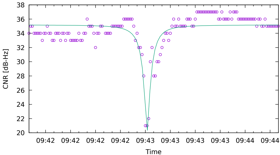
CNR fit for G17 on HuaweiP40 - drive 14 (DOY262)
