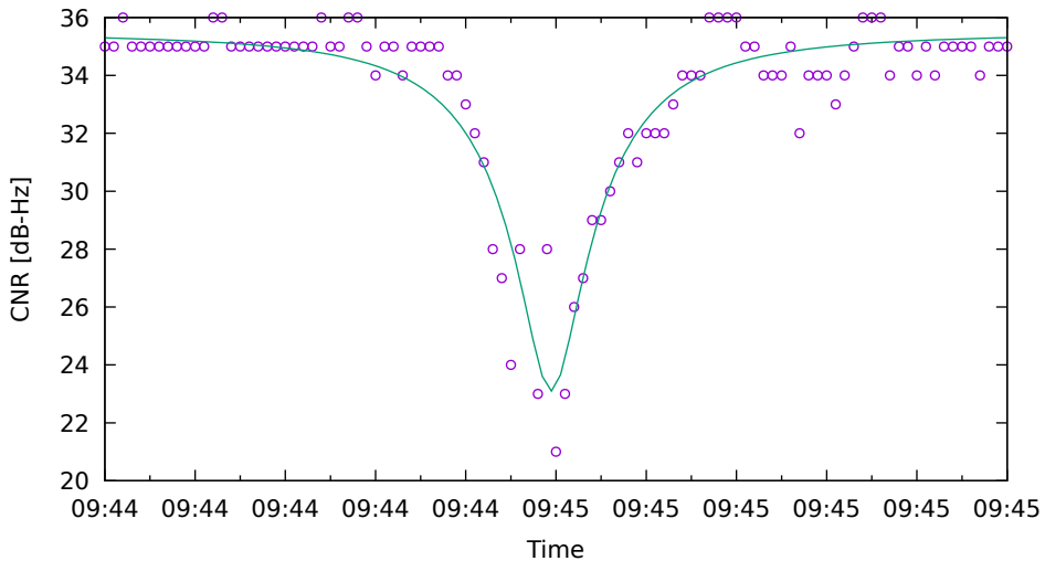
CNR fit for G17 on HuaweiP40 - drive 15 (DOY262)
