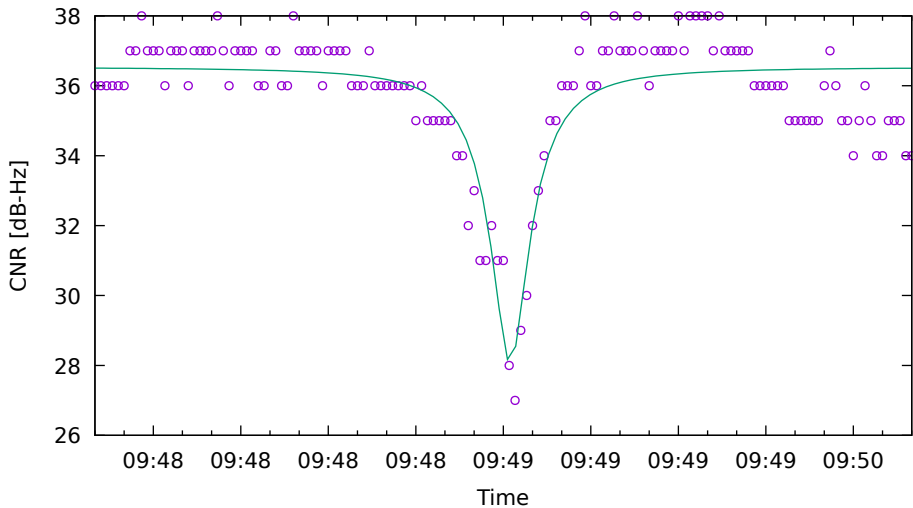
CNR fit for G17 on HuaweiP40 - drive 17 (DOY262)
