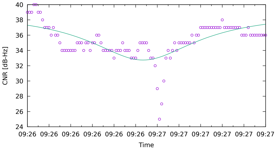
CNR fit for G17 on HuaweiP40 - drive 6 (DOY262)
