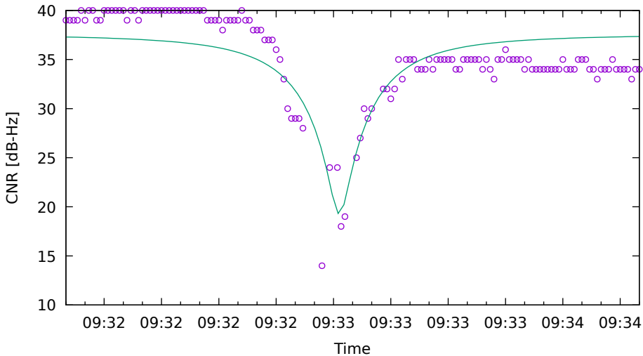
CNR fit for G17 on HuaweiP40 - drive 9 (DOY262)
