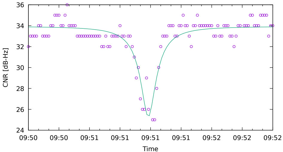
CNR fit for G19 on HuaweiP40 - drive 18 (DOY262)
