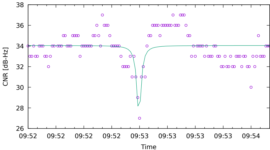
CNR fit for G19 on HuaweiP40 - drive 19 (DOY262)
