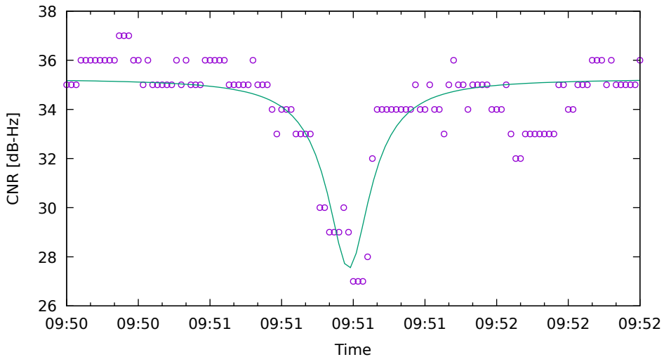
CNR fit for G21 on HuaweiP40 - drive 18 (DOY262)
