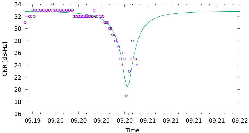
CNR fit for G21 on HuaweiP40 - drive 3 (DOY262)
