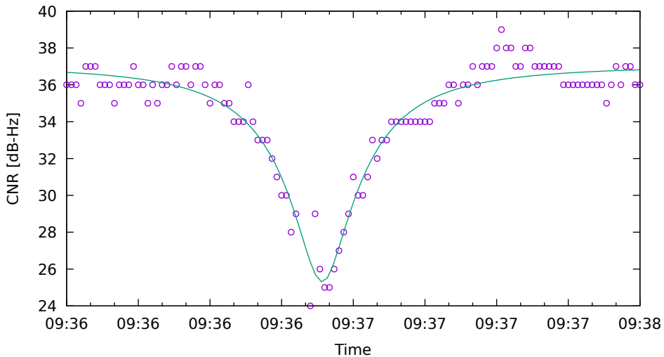
CNR fit for G22 on HuaweiP40 - drive 11 (DOY262)
