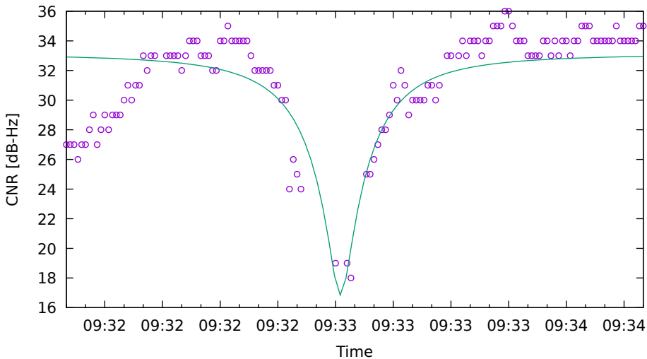
CNR fit for G22 on HuaweiP40 - drive 9 (DOY262)
