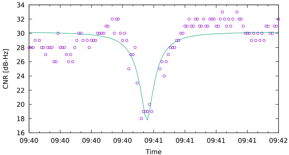
CNR fit for G31 on HuaweiP40 - drive 13 (DOY262)
