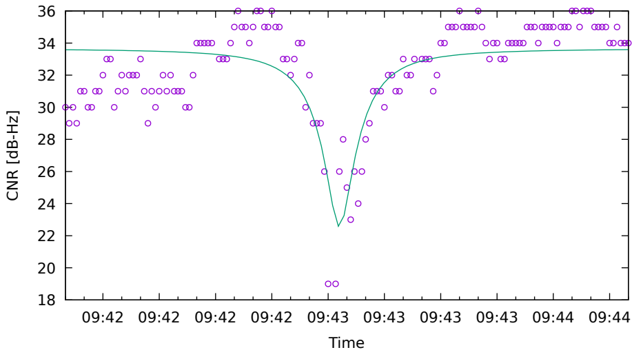
CNR fit for G31 on HuaweiP40 - drive 14 (DOY262)
