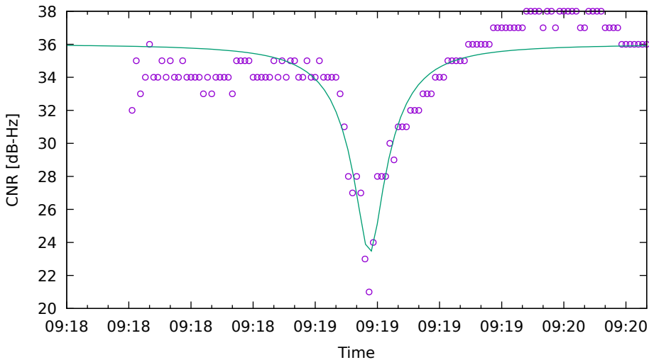
CNR fit for G31 on HuaweiP40 - drive 2 (DOY262)
