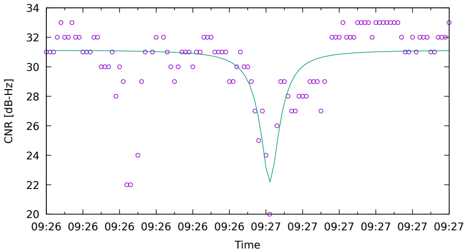
CNR fit for G31 on HuaweiP40 - drive 6 (DOY262)
