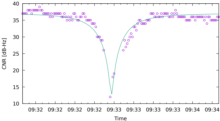
CNR fit for G31 on HuaweiP40 - drive 9 (DOY262)
