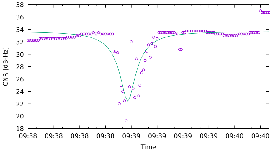
CNR fit for E05 on Xiaomi11T - drive 12 (DOY262)
