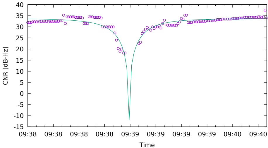
CNR fit for E09 on Xiaomi11T - drive 12 (DOY262)
