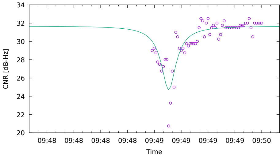
CNR fit for E09 on Xiaomi11T - drive 17 (DOY262)
