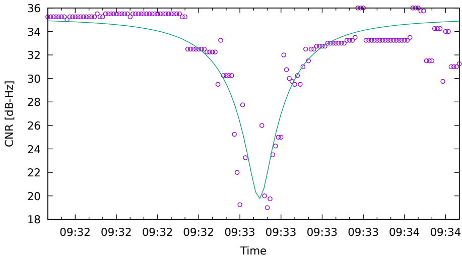
CNR fit for E09 on Xiaomi11T - drive 9 (DOY262)
