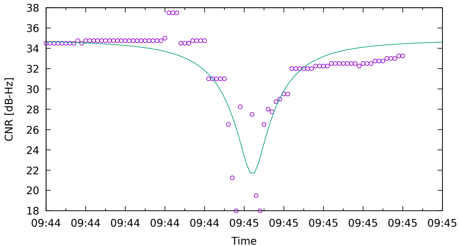
CNR fit for E34 on Xiaomi11T - drive 15 (DOY262)
