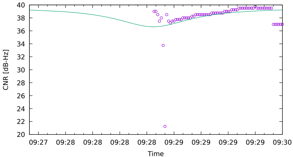
CNR fit for E34 on Xiaomi11T - drive 7 (DOY262)
