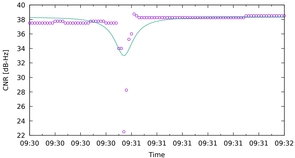
CNR fit for E34 on Xiaomi11T - drive 8 (DOY262)
