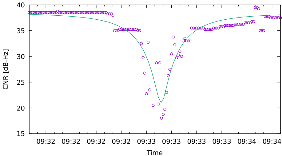
CNR fit for E34 on Xiaomi11T - drive 9 (DOY262)
