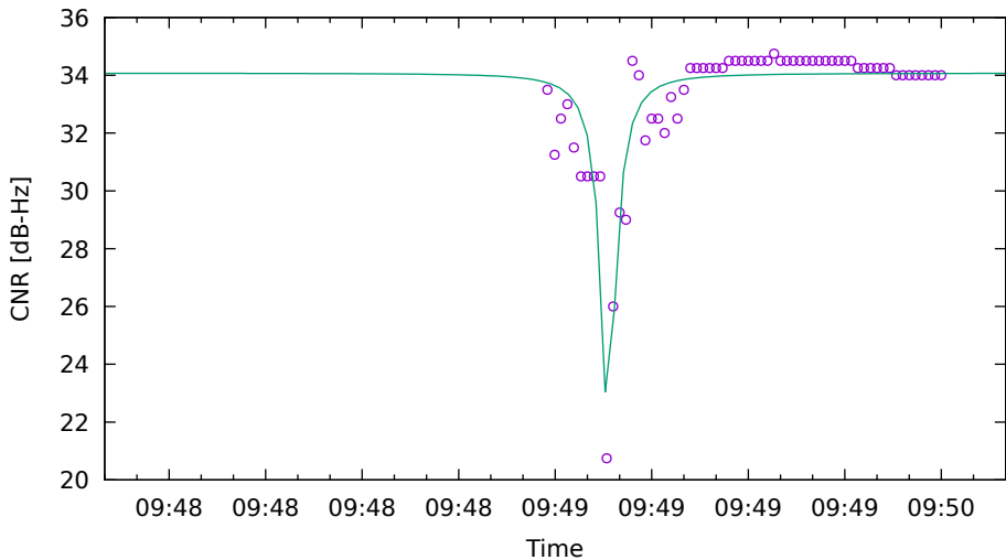
CNR fit for E36 on Xiaomi11T - drive 17 (DOY262)
