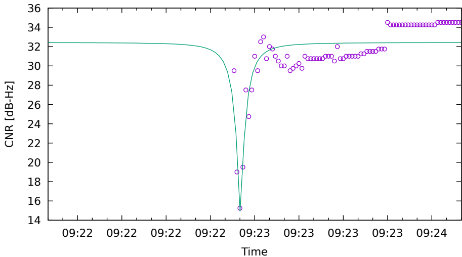
CNR fit for E36 on Xiaomi11T - drive 4 (DOY262)
