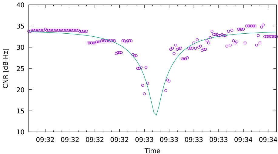
CNR fit for E36 on Xiaomi11T - drive 9 (DOY262)
