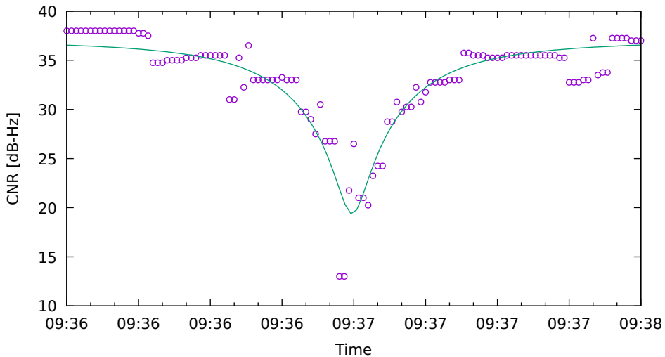
CNR fit for G01 on Xiaomi11T - drive 11 (DOY262)
