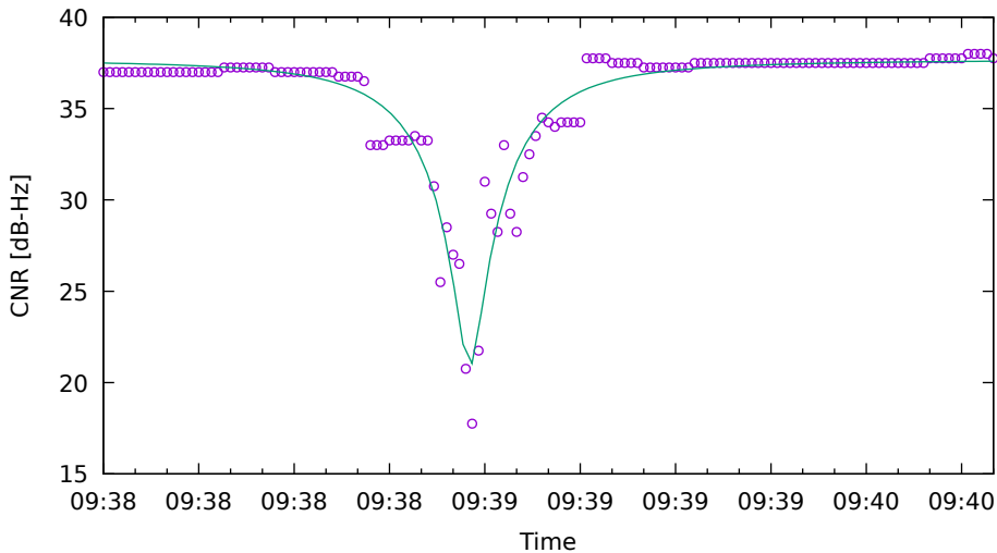
CNR fit for G01 on Xiaomi11T - drive 12 (DOY262)
