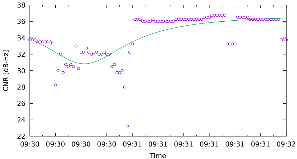
CNR fit for G01 on Xiaomi11T - drive 8 (DOY262)
