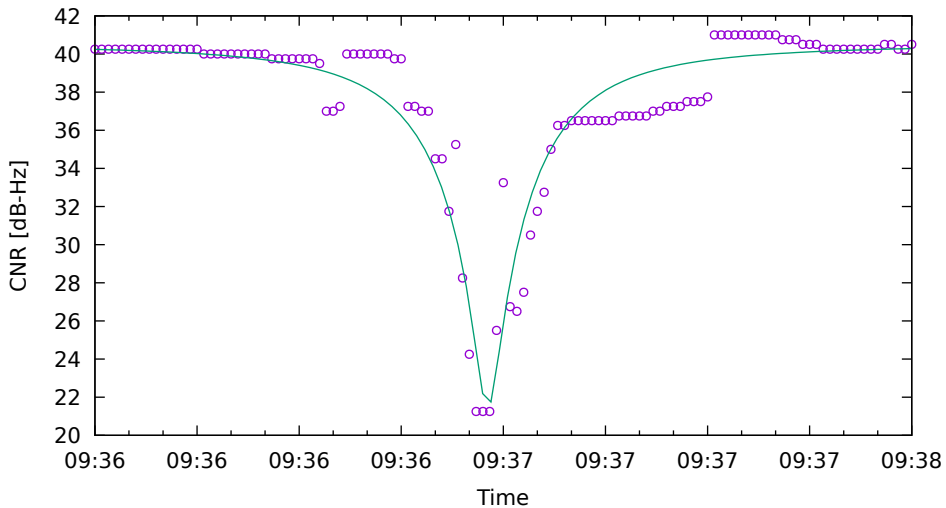
CNR fit for G03 on Xiaomi11T - drive 11 (DOY262)
