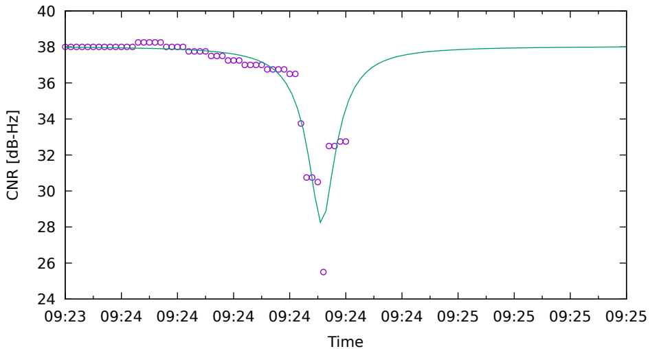
CNR fit for G03 on Xiaomi11T - drive 5 (DOY262)
